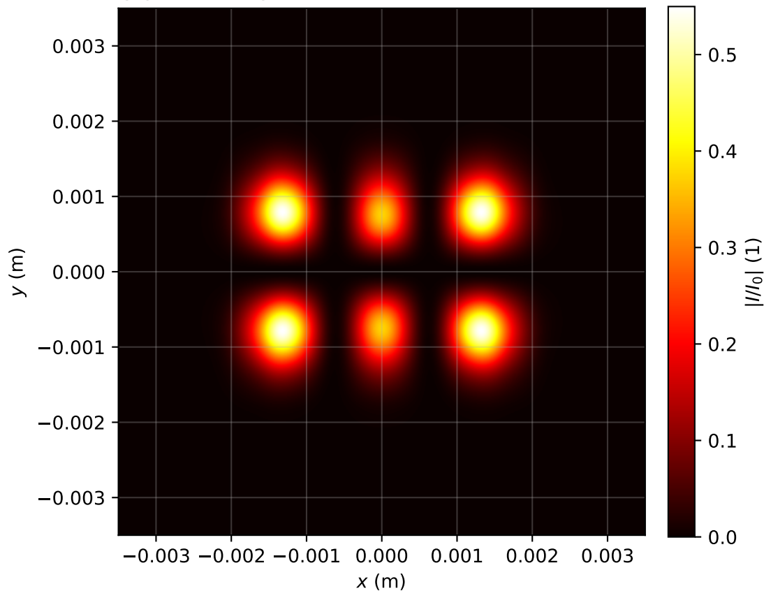
Intensity profile I(x, y, z = 2.627)/I_0 , P_{in}=2.0P_{cr} , artificial time
